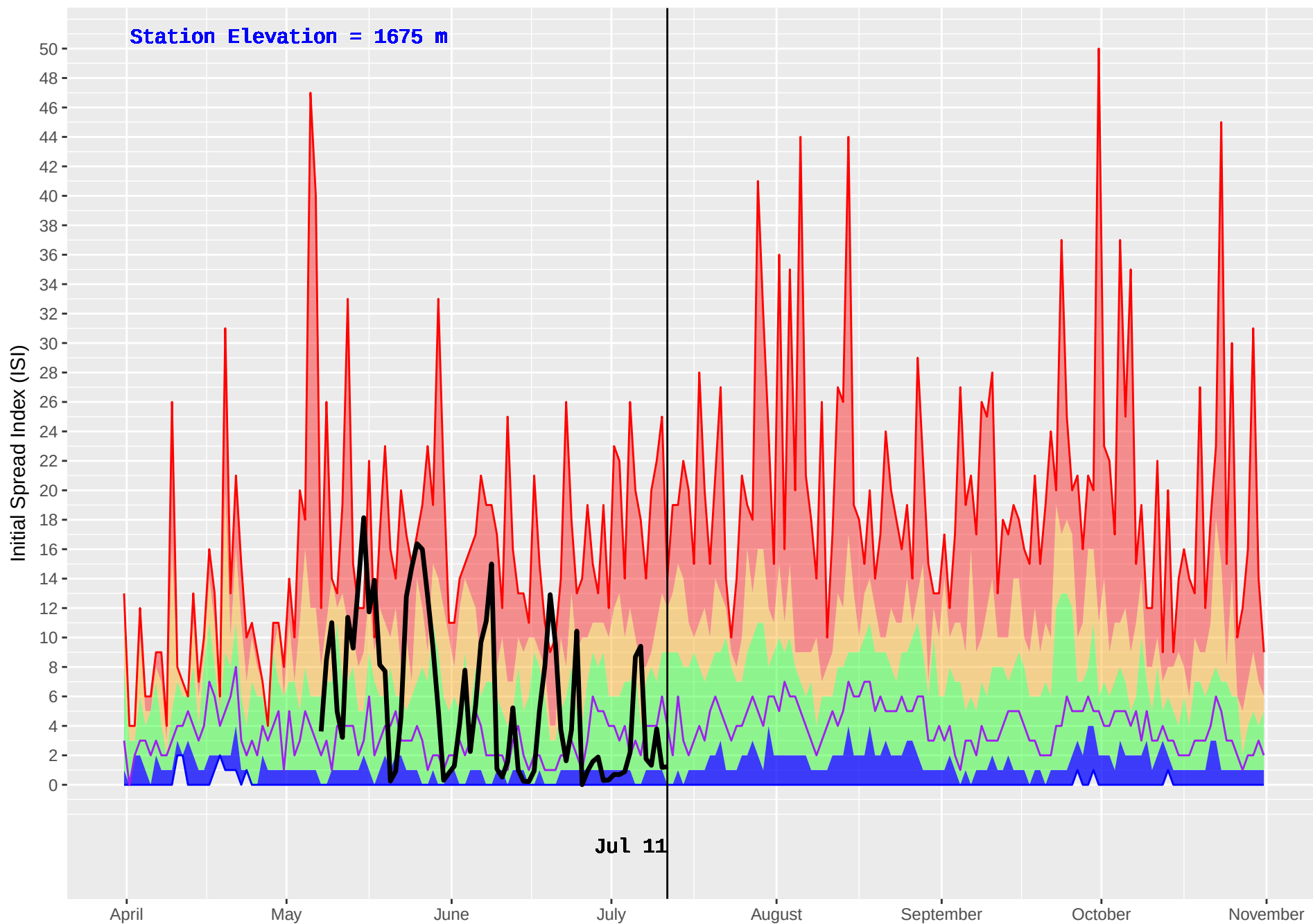
GASPARD (222) : Historical (1992–2016) and Current (2018) Noon Initial Spread Index (ISI)
